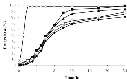
Fig 2: Drug release tramadol tablets containing Carbopol 974P. Key: ■ = F5, ▲ = F6, □ = F7, x = F8, and ● = F9, compared standard (◇); n = 3
