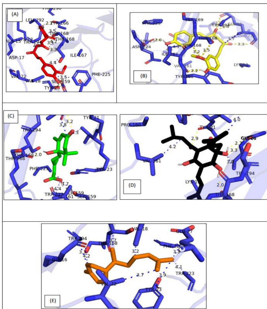
Figure 1: (A) Fibrinogen with curcumin, (B) Fibrinogen with demethoxycurcumin, (C) Fibrinogen with abscisic Acid (D) Fibrinogen with humulone and (E) Fibrinogen with zingiberene. Blue bonds represent nonpolar interactions, and yellow bonds represent polar interactions
