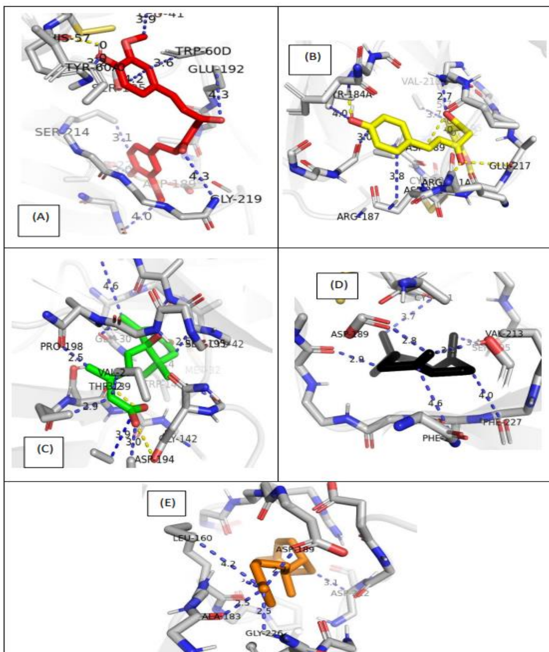
Figure 2: (A) Prothrombin with curcumin, (B) Prothrombin with demethoxycurcumin, (C) Prothrombin with abscisic Acid (D) Prothrombin with humulone and (E) Prothrombin with zingiberene. Blue bonds represent non-polar interactions, and yellow bonds represent polar interactions
