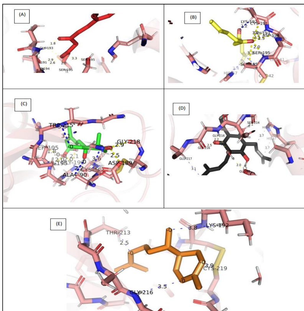
Figure 4: (A) Factor Xla antecedent with curcumin, (B) Factor Xla with demethoxycurcumin, (C) Factor Xla with absciscic Acid (D) Factor Xla with humulone and (E) Factor Xla with zingiberene. Blue bonds represent non-polar interactions, and yellow bonds represent polar interactions
