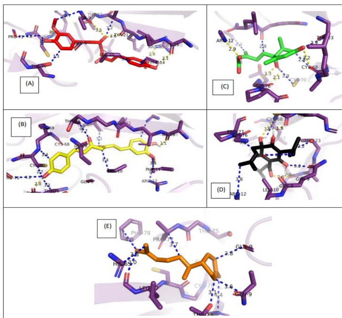
Figure 3: (A) Hageman factor with curcumin, (B) Hageman factor with demethoxycurcumin, (C) Hageman factor with absciscic Acid (D) Hageman factor with humulone and (E) Hageman factor with zingiberene. Blue bonds represent non-polar interactions, and yellow bonds represent polar interactions
