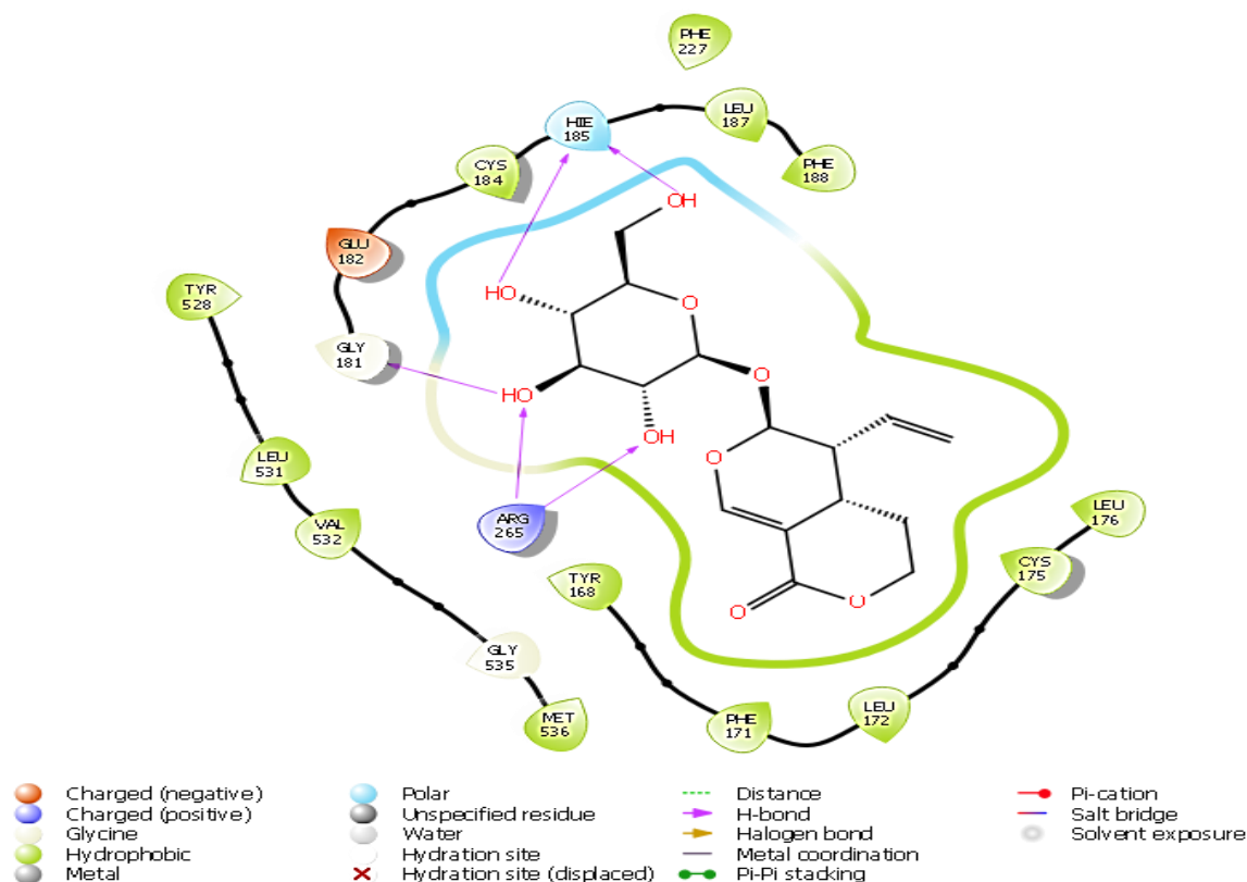
Figure 1: 2D Interaction of Sweroside with amino acid residue within the binding site of Plasmodium falciparum dihydroorotate dehydrogenase protein
