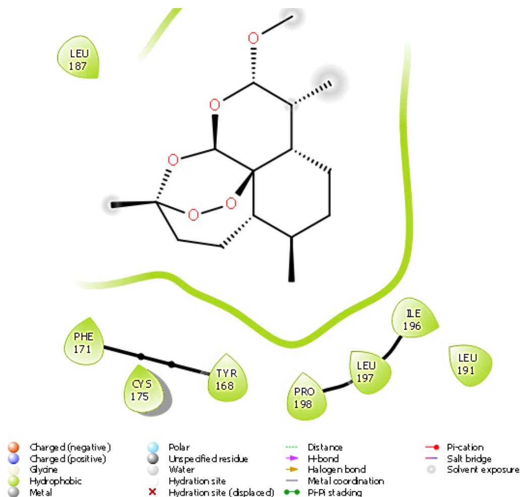
Figure 6: 2D Interaction of Artemether with amino acid residue within the binding site of Plasmodium falciparum dihydroorotate dehydrogenase protein
