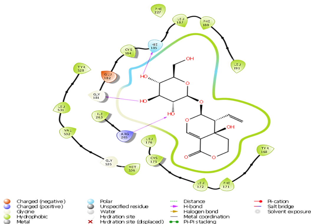
Figure 3: 2D Interaction of Swertiamarin with amino acid residue within the binding site of Plasmodium falciparum dihydroorotate dehydrogenase protein
