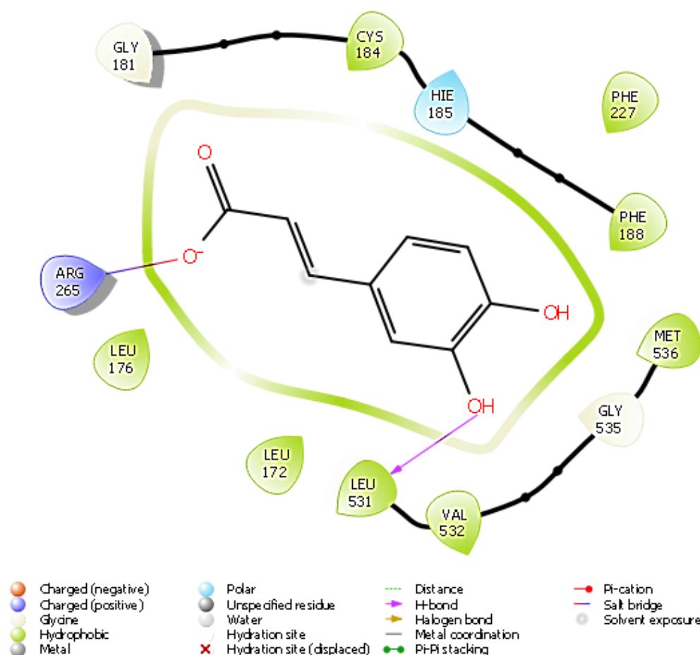
Figure 5: 2D Interaction of Caffeic acid with amino acid residue within the binding site of Plasmodium falciparum dihydroorotate dehydrogenase protein
