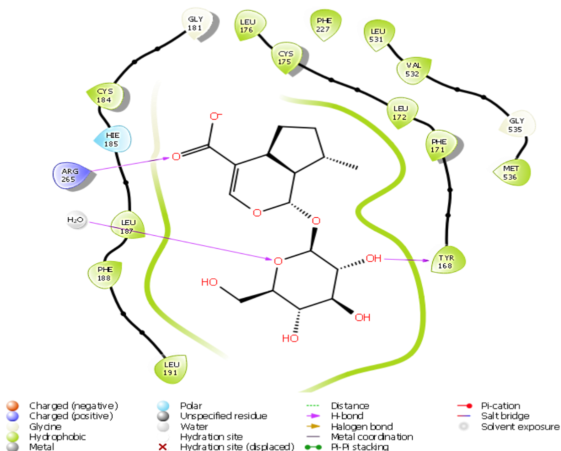
Figure 2: 2D Interaction of 7-Deoxyloganic acid with amino acid residue within the binding site of Plasmodium falciparum dihydroorotate dehydrogenase protein
