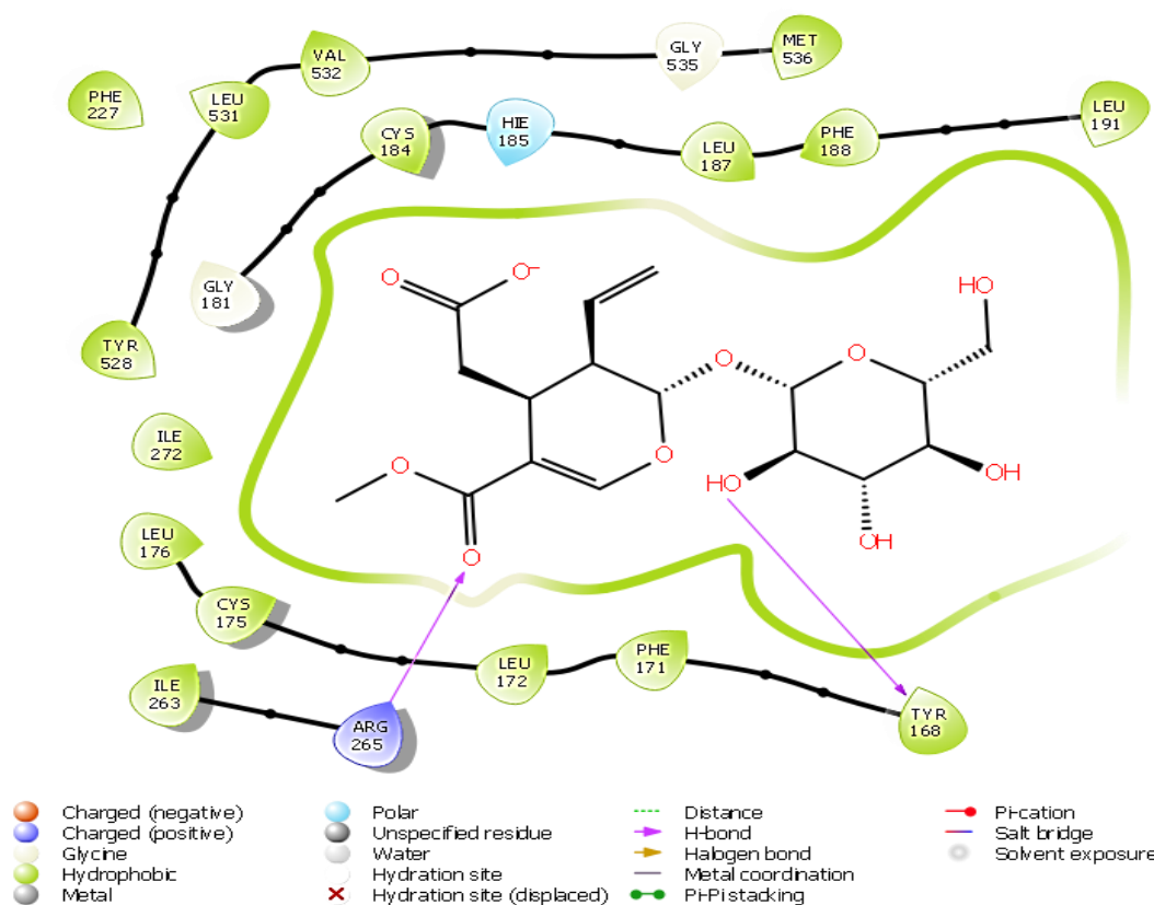
Figure 4: 2D Interaction of Secologanoside methyl ester with amino acid residue within the binding site of Plasmodium falciparum dihydroorotate dehydrogenase protein
